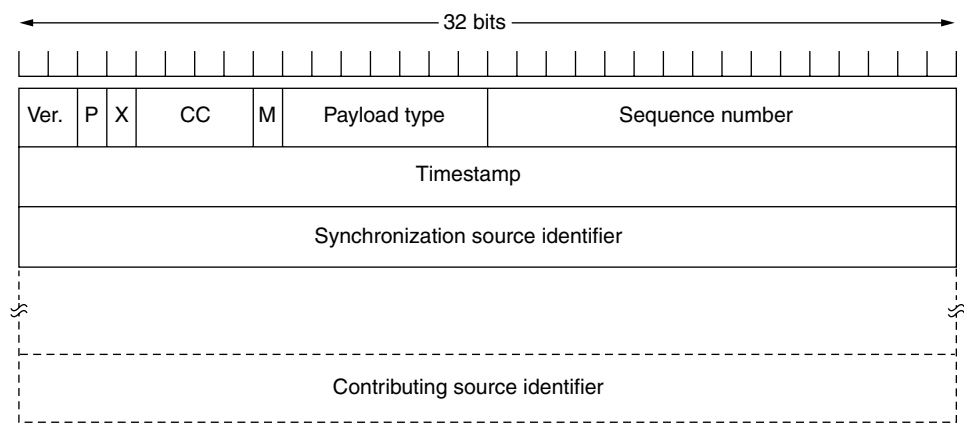
Figure 6-31. The RTP header.
